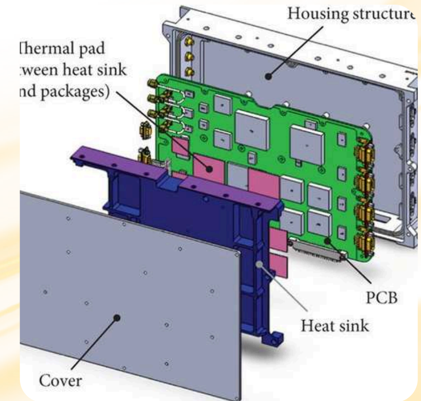
Heat Sink Cooling
